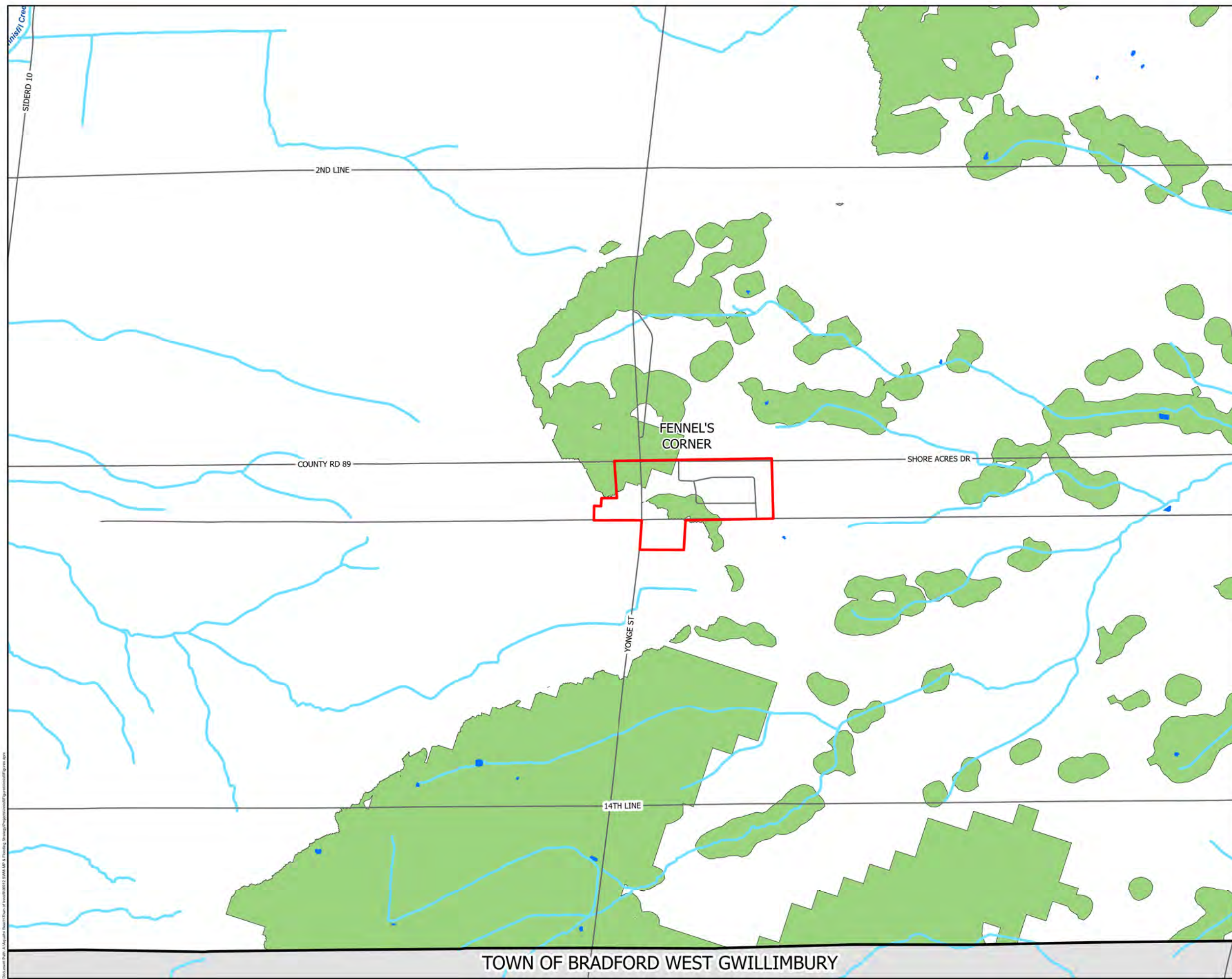
Figure 4.3 Significant Groundwater Recharge Areas (7 of 9)
