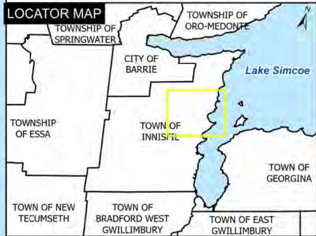
Figure 4.3 Significant Groundwater Recharge Areas (2 of 9)
