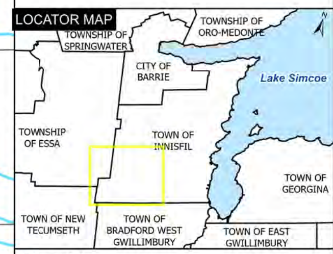
Figure 4.3 Significant Groundwater Recharge Areas (9 of 9)
