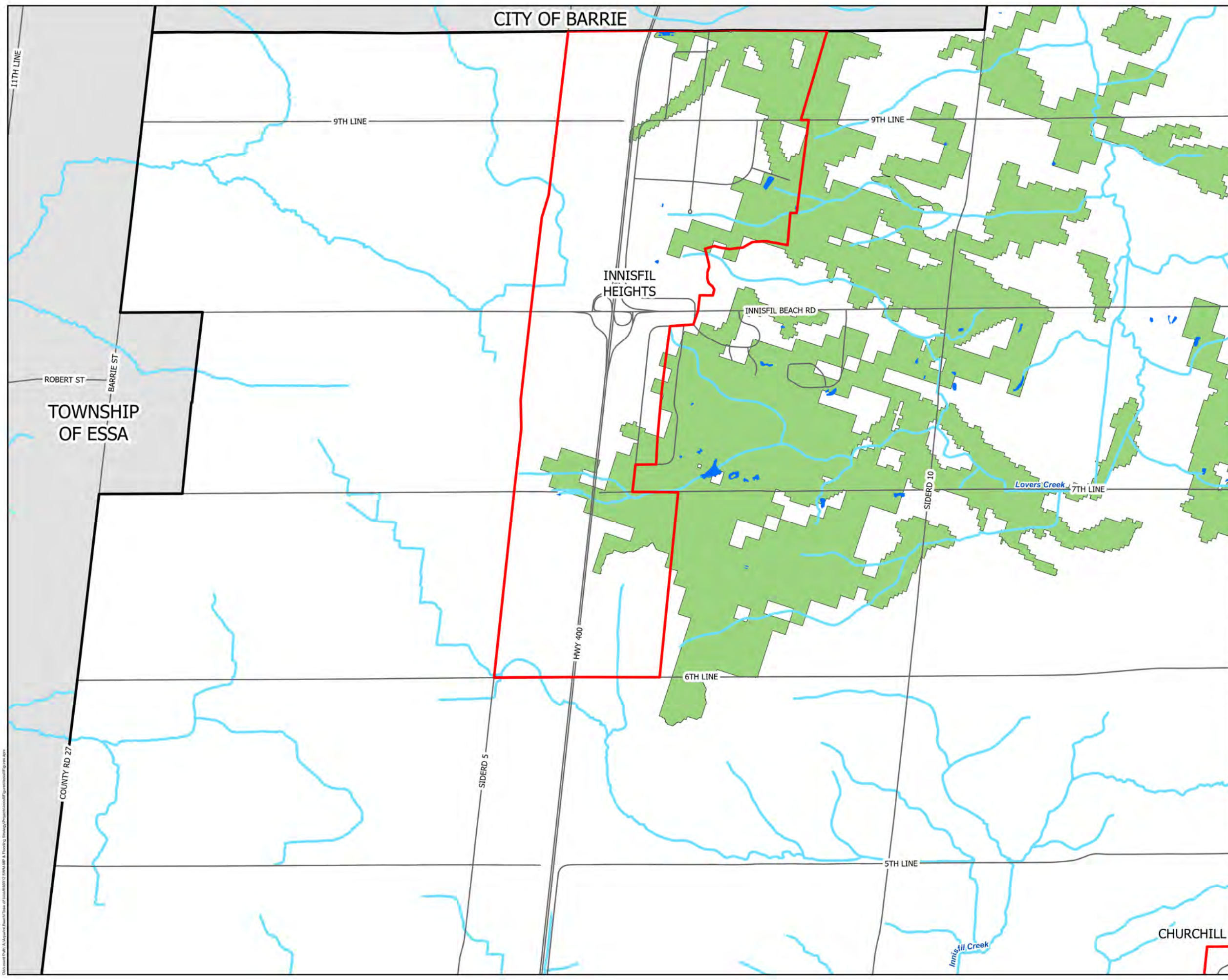
Figure 4.3 Significant Groundwater Recharge Areas (8 of 9)
