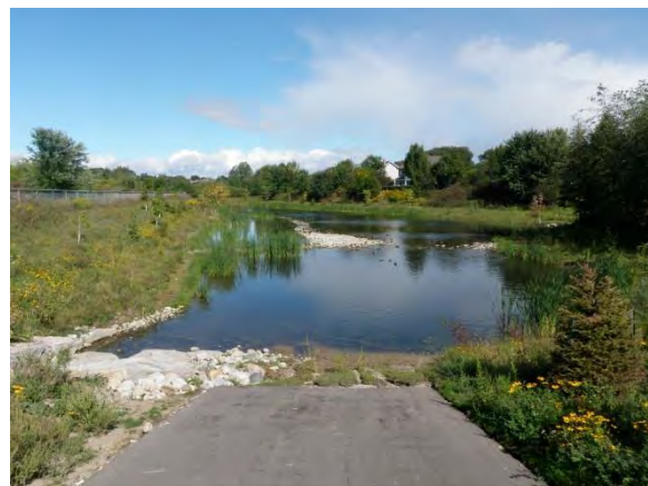
Hybrid wet pond/ wetland
