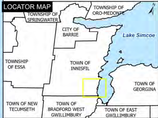
Figure 4.3 Significant Groundwater Recharge Areas (4 of 9)
