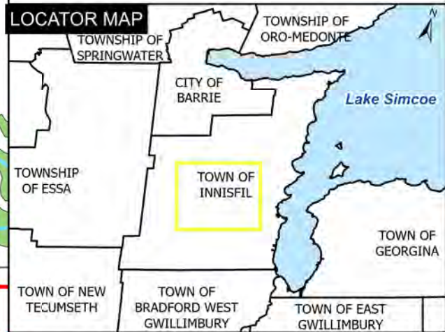
Figure 4.3 Significant Groundwater Recharge Areas (6 of 9)
