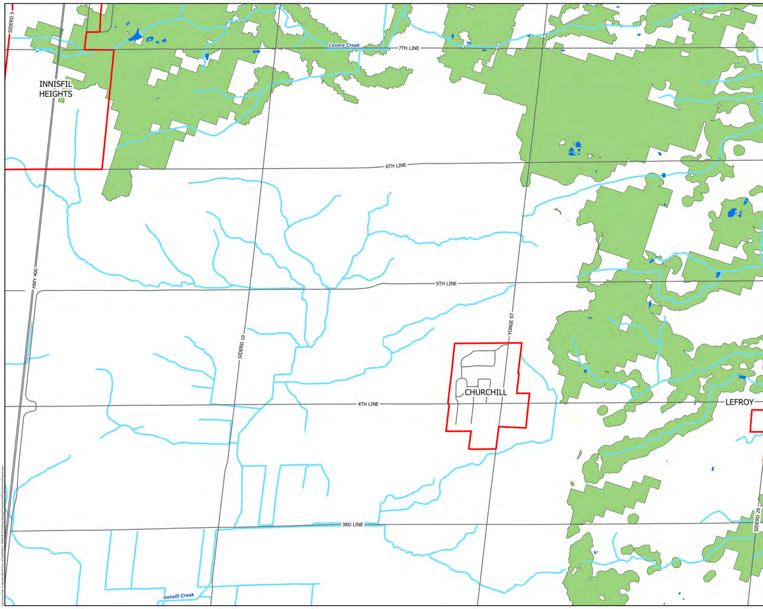
Figure 4.3 Significant Groundwater Recharge Areas (6 of 9)
