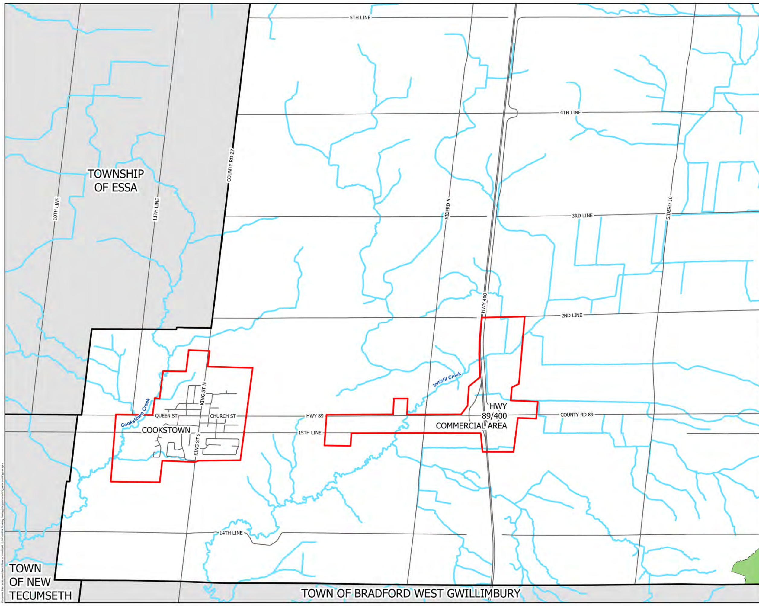
Figure 4.3 Significant Groundwater Recharge Areas (9 of 9)
