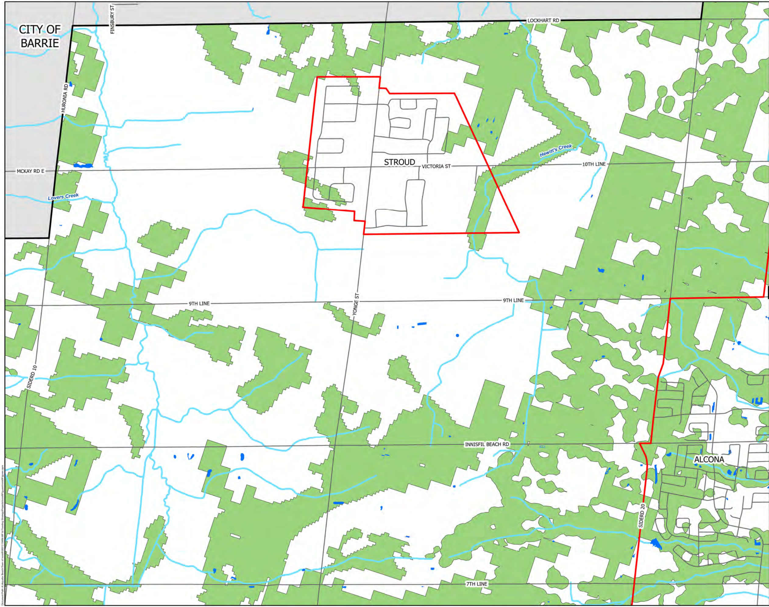
Figure 4.3 Significant Groundwater Recharge Areas (5 of 9)
