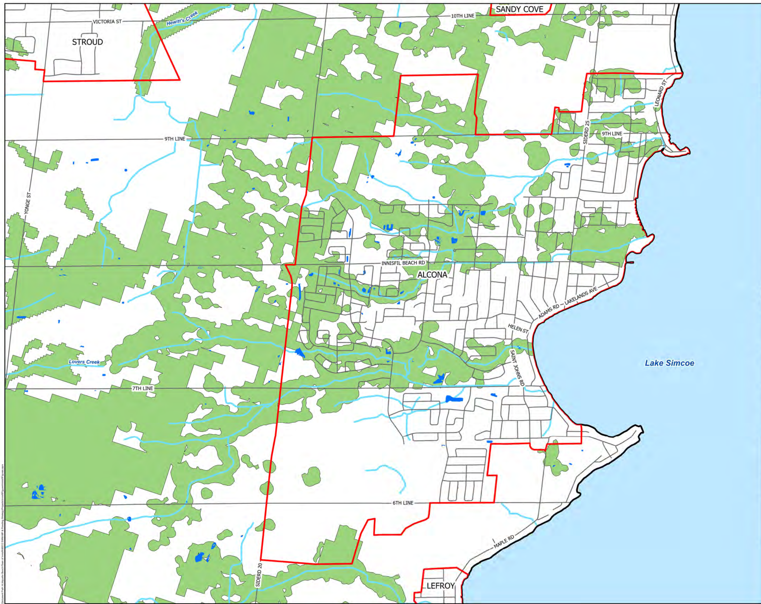
Figure 4.3 Significant Groundwater Recharge Areas (2 of 9)
