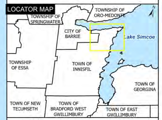
Figure 4.3 Significant Groundwater Recharge Areas (1 of 9)
