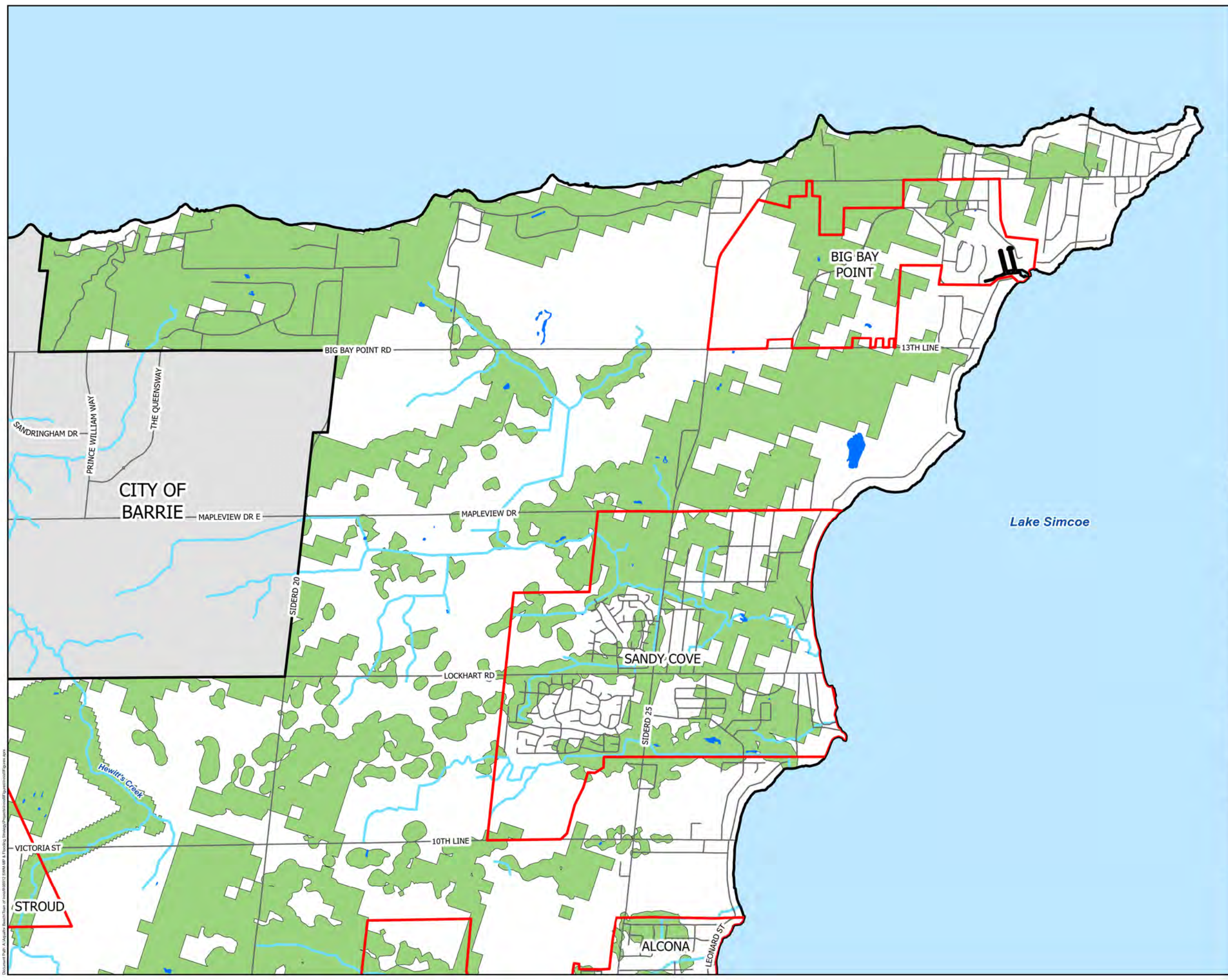
Figure 4.3 Significant Groundwater Recharge Areas (1 of 9)
