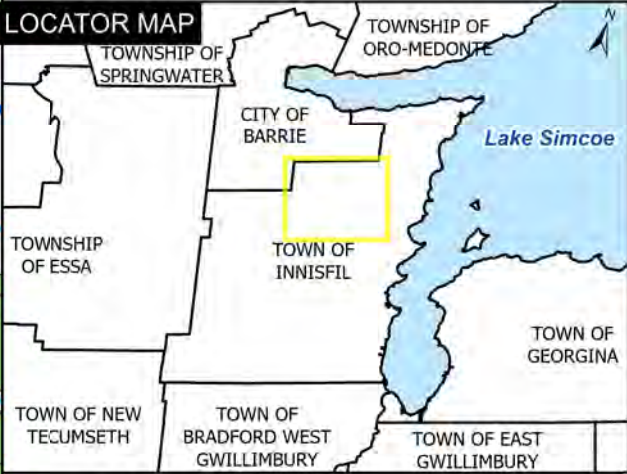
Figure 4.3 Significant Groundwater Recharge Areas (5 of 9)
