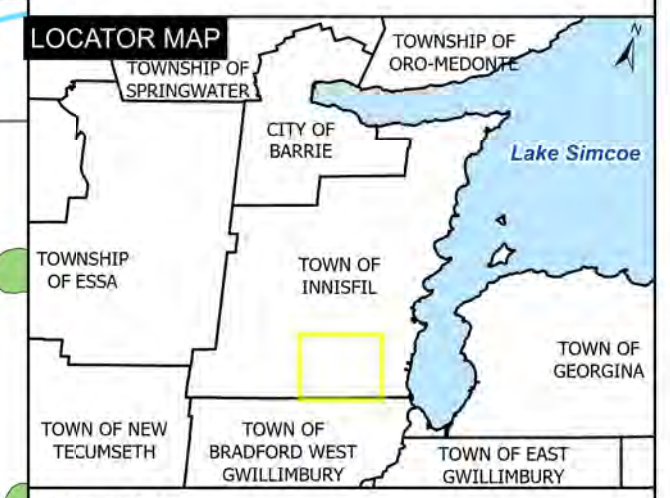
Figure 4.3 Significant Groundwater Recharge Areas (7 of 9)
