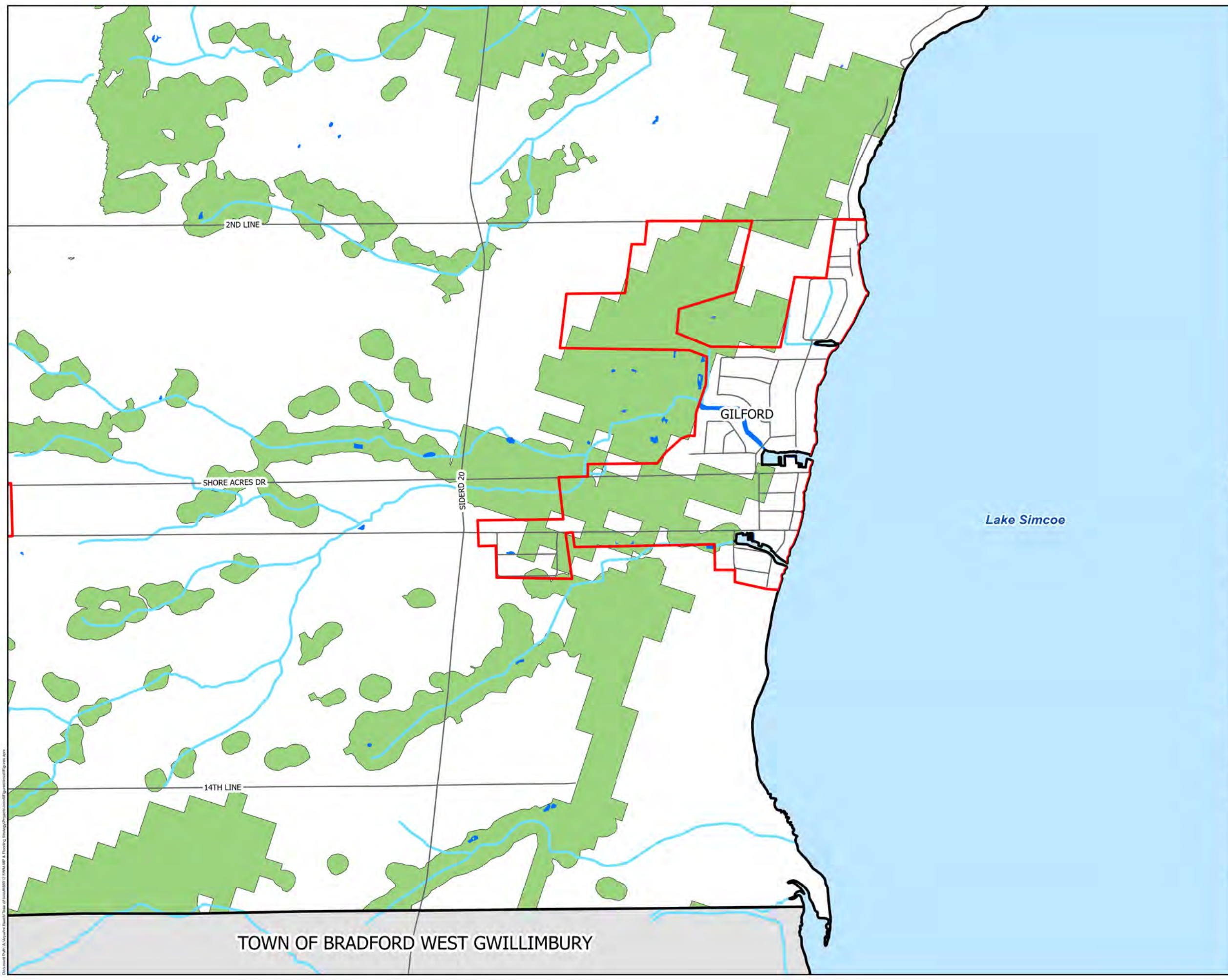
Figure 4.3 Significant Groundwater Recharge Areas (4 of 9)
