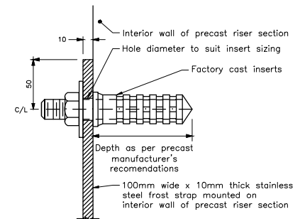
FROST STRAP SECTION
