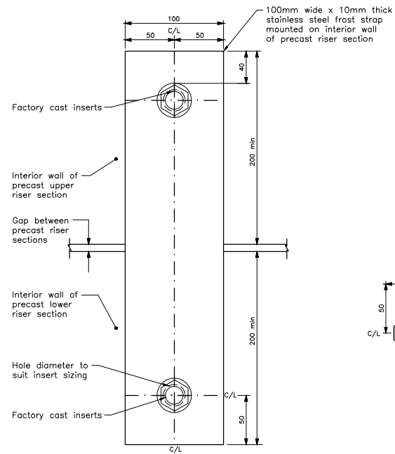
FROST STRAP ANCHORED TO INTERNAL WALL
