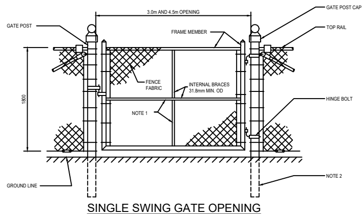
SINGLE SWING GATE OPENING
