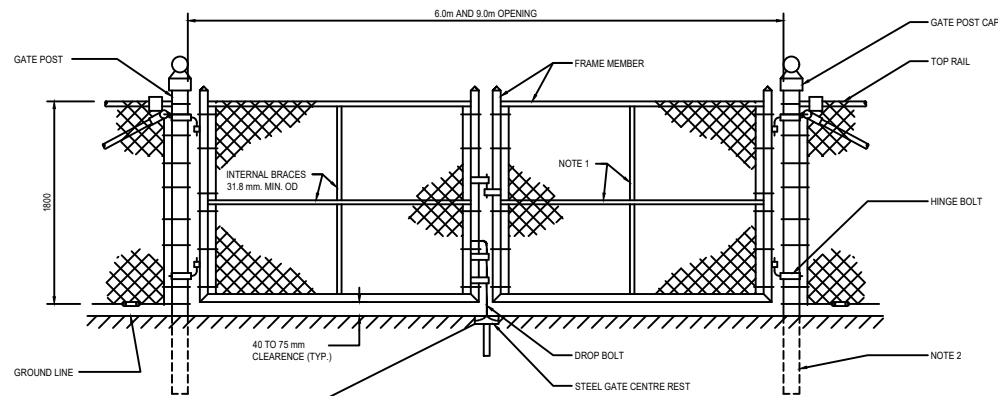
DOUBLE SWING GATE OPENING
